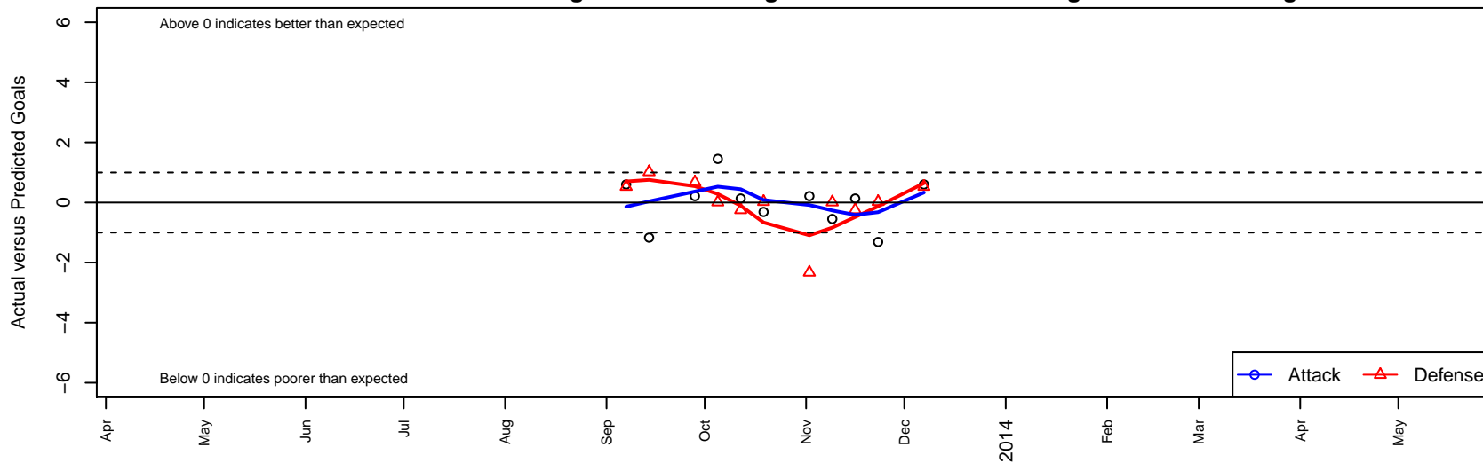
Highlands SC Thunderhawks B00 Dots are actual minus expected GF (blue circles) and GA (red triangles). Blue line is smoothed change in attack strength. Red is smoothed change in defense strength.
